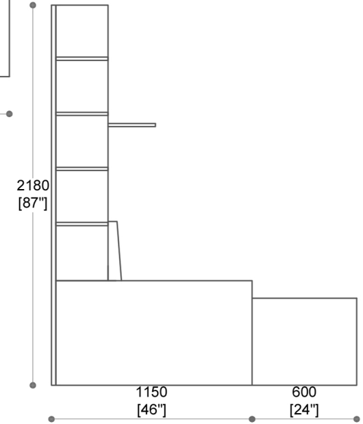
SECTION -B-B'
