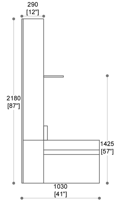
SECTION - B-B'
